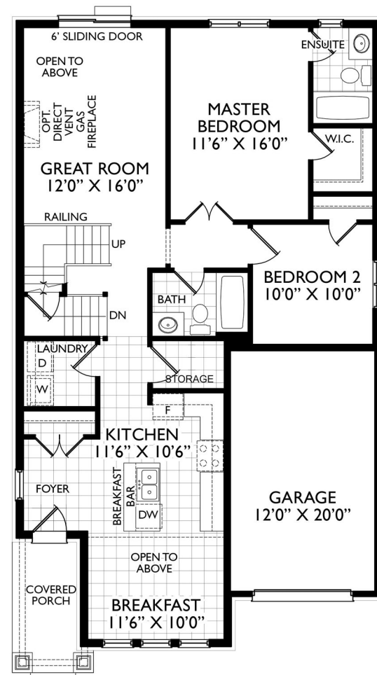
GROUND PLAN EL. 'A'
